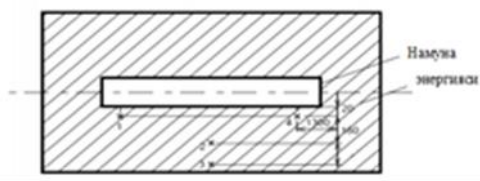
Figure 2. Installation diagram of thermocouples in the cross section of the furnace.
