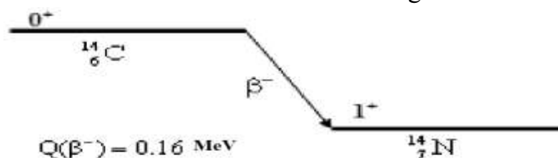
1-rasm. ^{14}\text{C} -izotopining parchalanish sxemasi.
